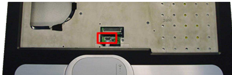
Fig. 11 Disconnecting touchpad flat cable
