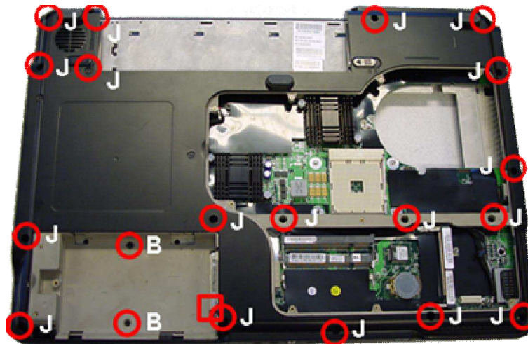
Fig. 23 The bottom base assembly.
