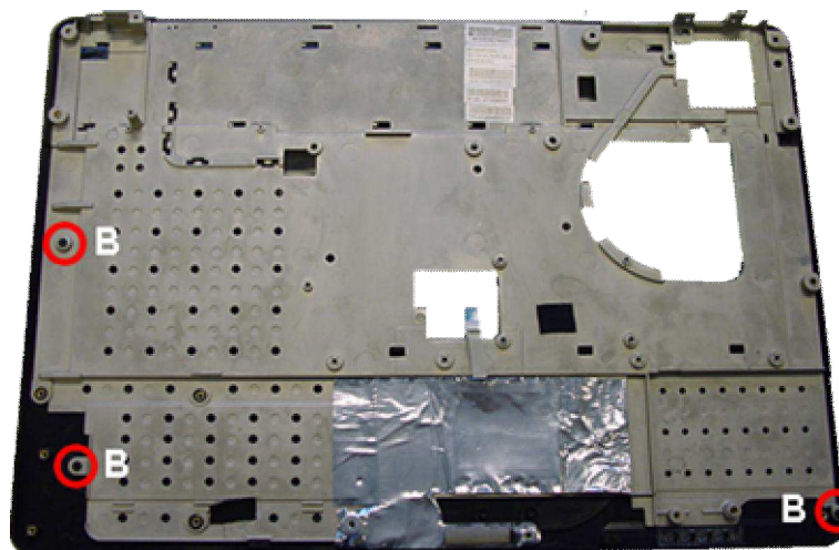
Fig. 28 Removing the heat plate.
