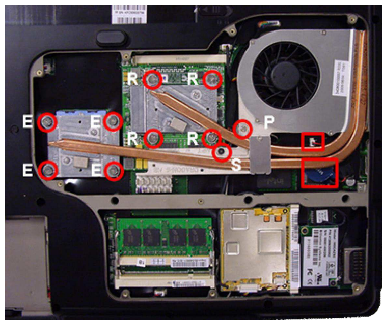
Fig. 6 Removing the heat sink.
