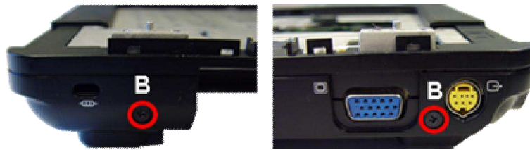
Fig. 24 The screws at the bottom base rear.
