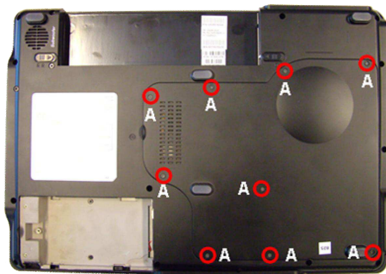
Fig. 4 Removing the bottom panel.
