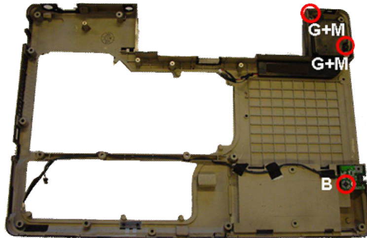
Fig. 25 The bottom cover.
