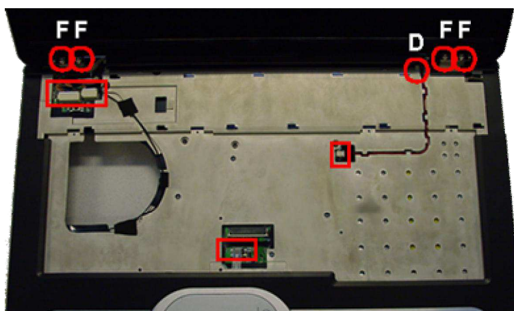
Fig. 13 Lid switch and hinges.
