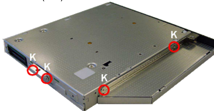
Fig. 21 The screws of the optical disk drive brackets.
