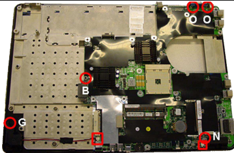
Fig. 26 The main board and speakers.
