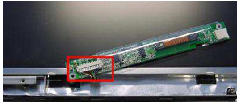
Fig. 16 LCD inverter backlight connector.
