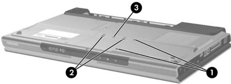
Black Phillips M2.0x5.0 Screw Locations
