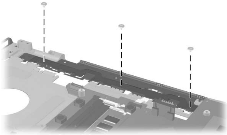
Phillips M1.5×2.0 Screw Locations
