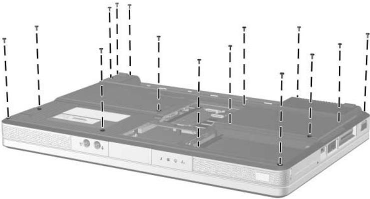
Phillips M2.0x8.5 Screw Locations
