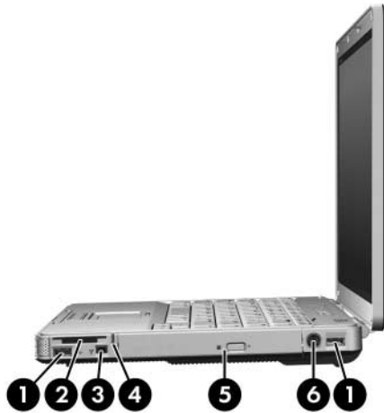
Right-Side Components, HP Compaq nx4820 and Compaq Presario V2400
