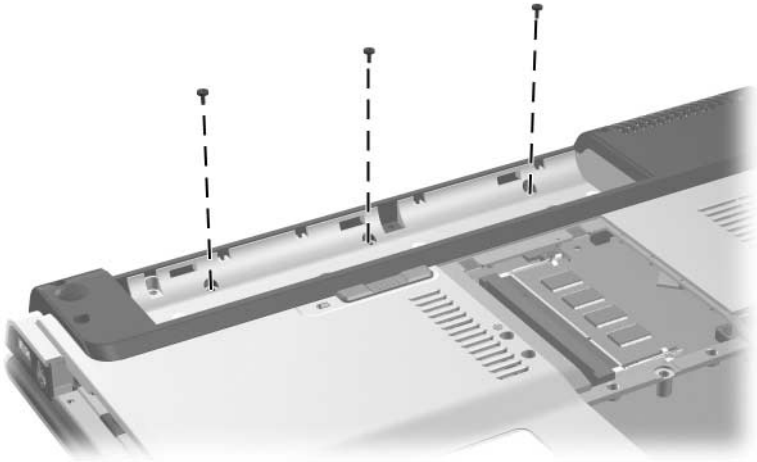
Removing the Switch Cover Screws, HP Pavilion dv1400 Models Only
