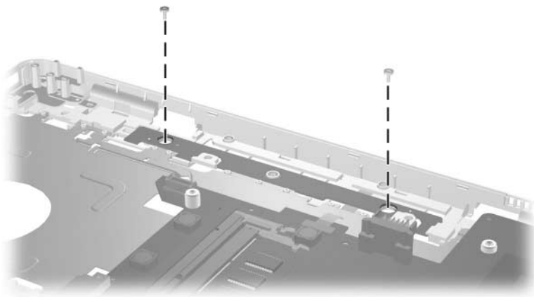
Phillips M2.0×3.0 Screw Locations
