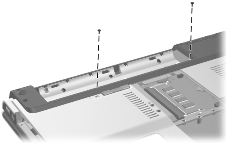
Silver Phillips M2.0×5.0 Screw Locations
