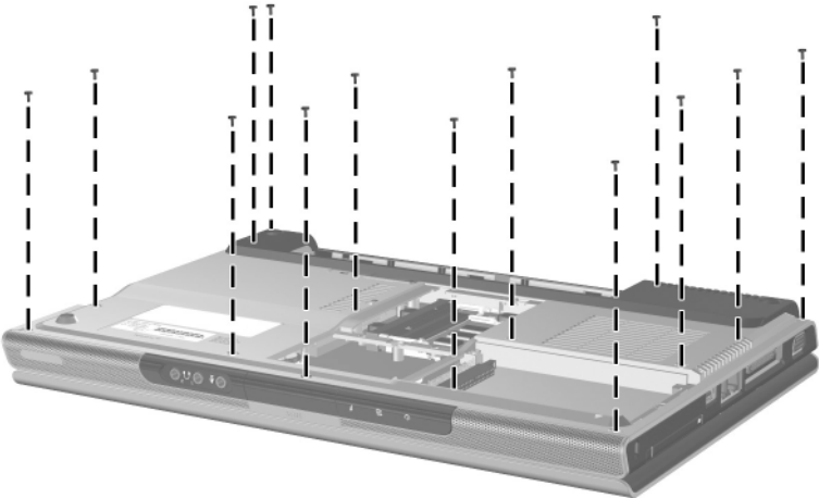
Phillips M2.0×8.5 Screw Locations
