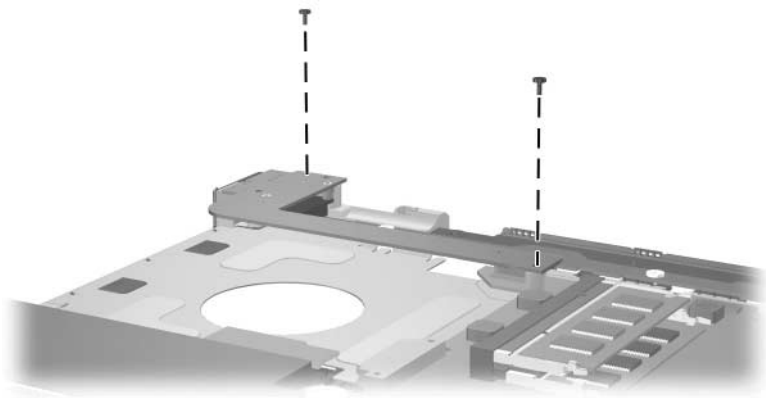
Silver Phillips M2.0×5.0 Screw Locations
