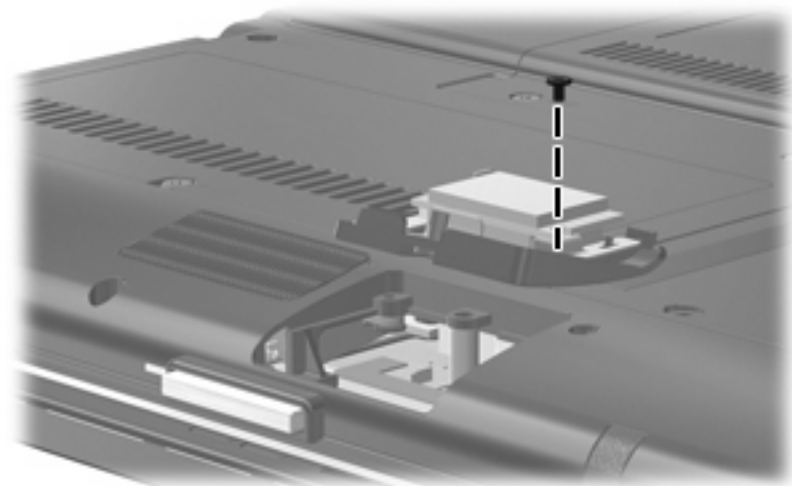
Where used: 1 screw that secures the Bluetooth module to the Bluetooth module compartment cover
