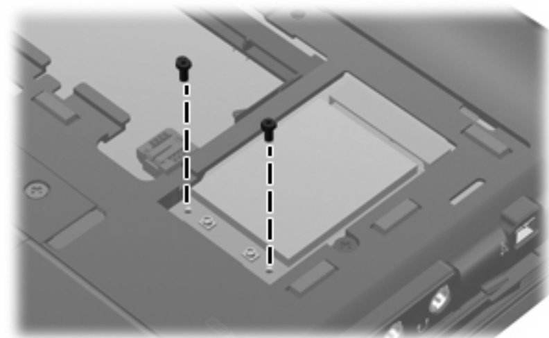
Where used: 2 screws that secure the WLAN module to the base enclosure
