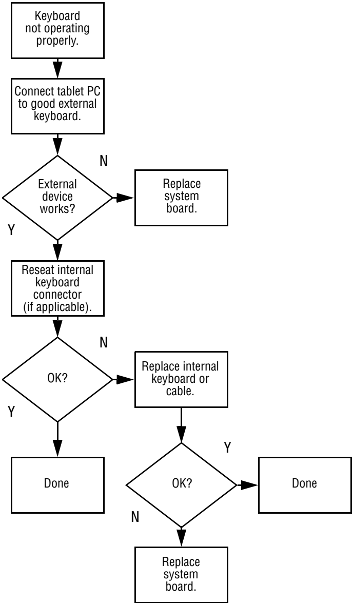
Flowchart 2.18—Nonfunctioning Keyboard
