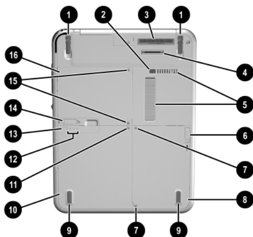
Figure 1-8. Bottom Components
