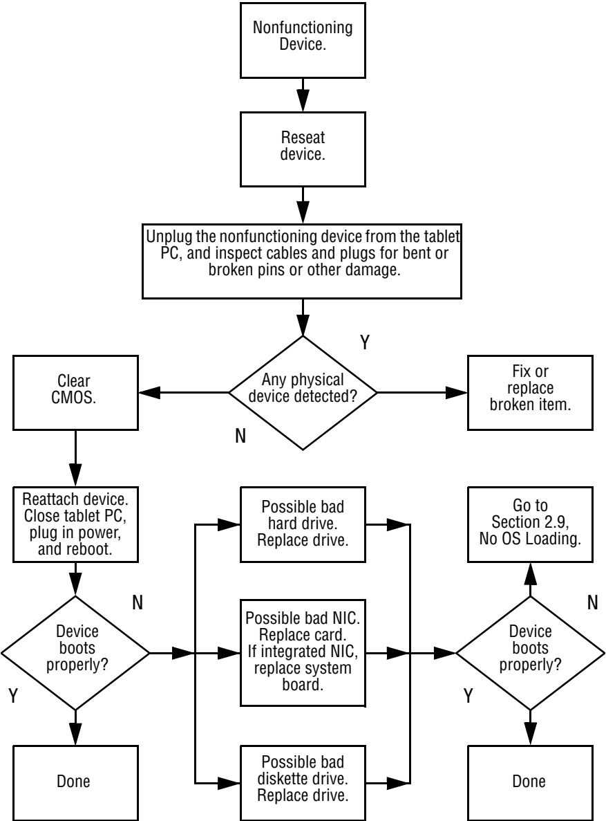
Flowchart 2.17—Nonfunctioning Device
