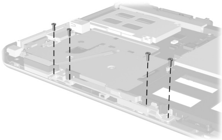
Figure C-4. Torx M2.5 × 7.0 Screw Locations
