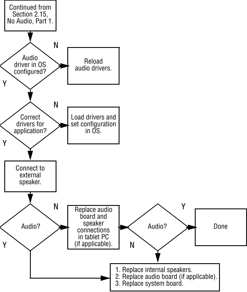
Flowchart 2.16—No Audio, Part 2
