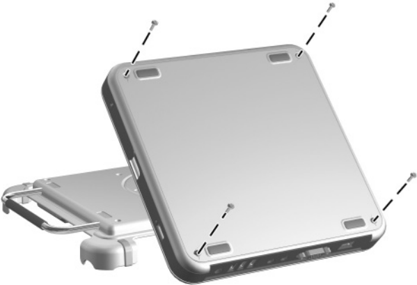
Figure C-5. Torx M2.5 × 7.0 Screw Locations
